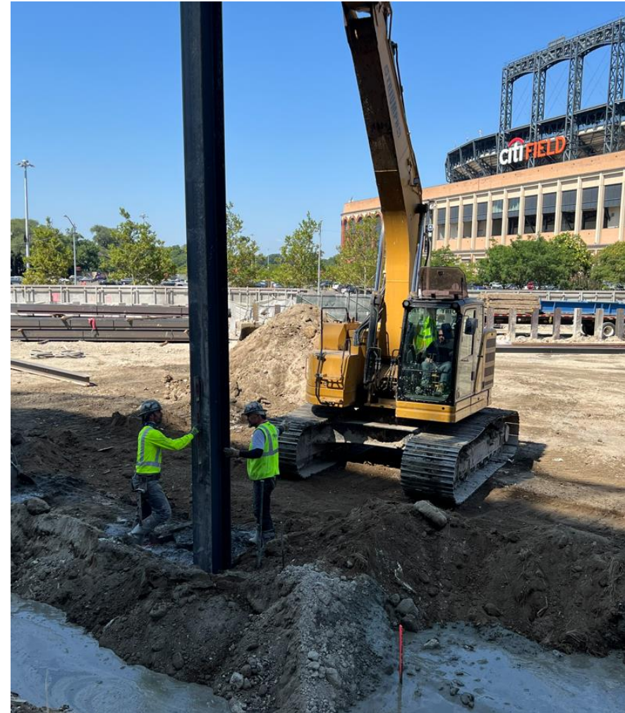
Triangle Open Space – Support-of-Excavation Installation
