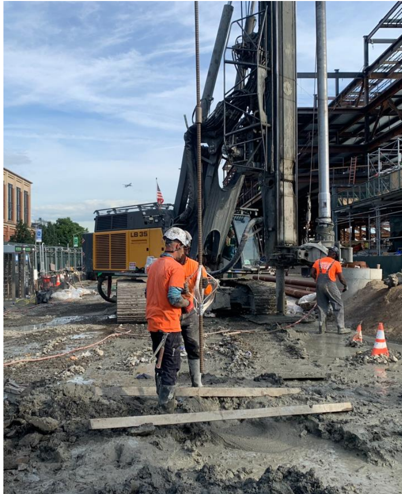
Stadium Open Space – Foundation Pile Installation
