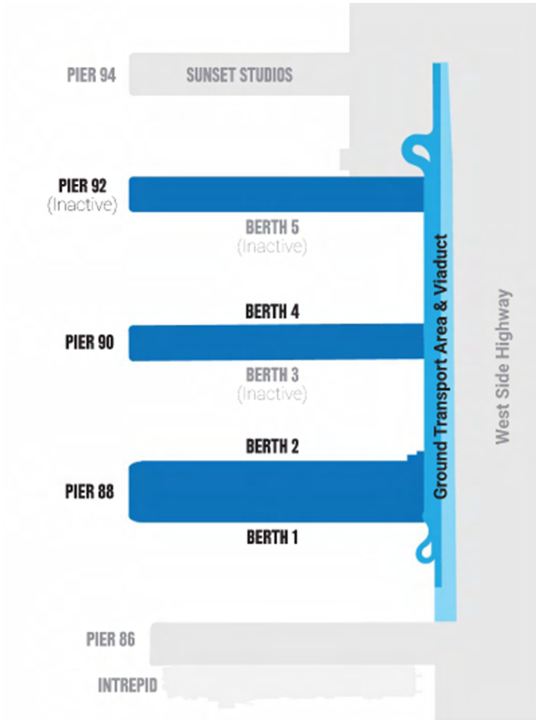
Figure 1-2: Berth Layout at MCT in its Current Configuration
