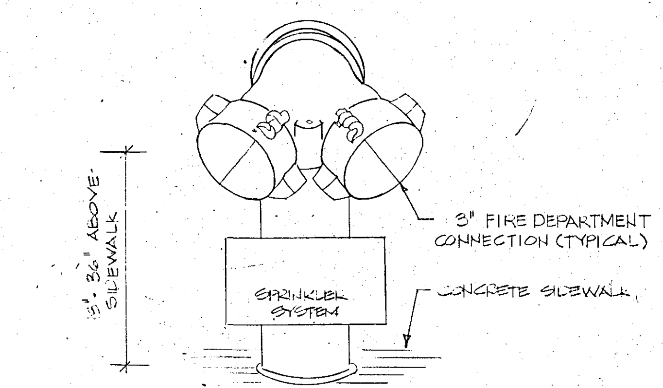
TYPICAL FIRE DEPARTMENT CONNECTION DETAIL N.T.S.
