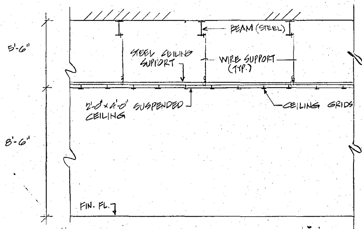
TYPICAL HUNG CEILING ELEVATION (DINING RM. & KITCHEN AREA) N.T.S.
