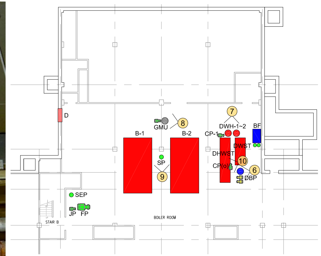
KEYPLAN (Partial Basement Floor Plan)
