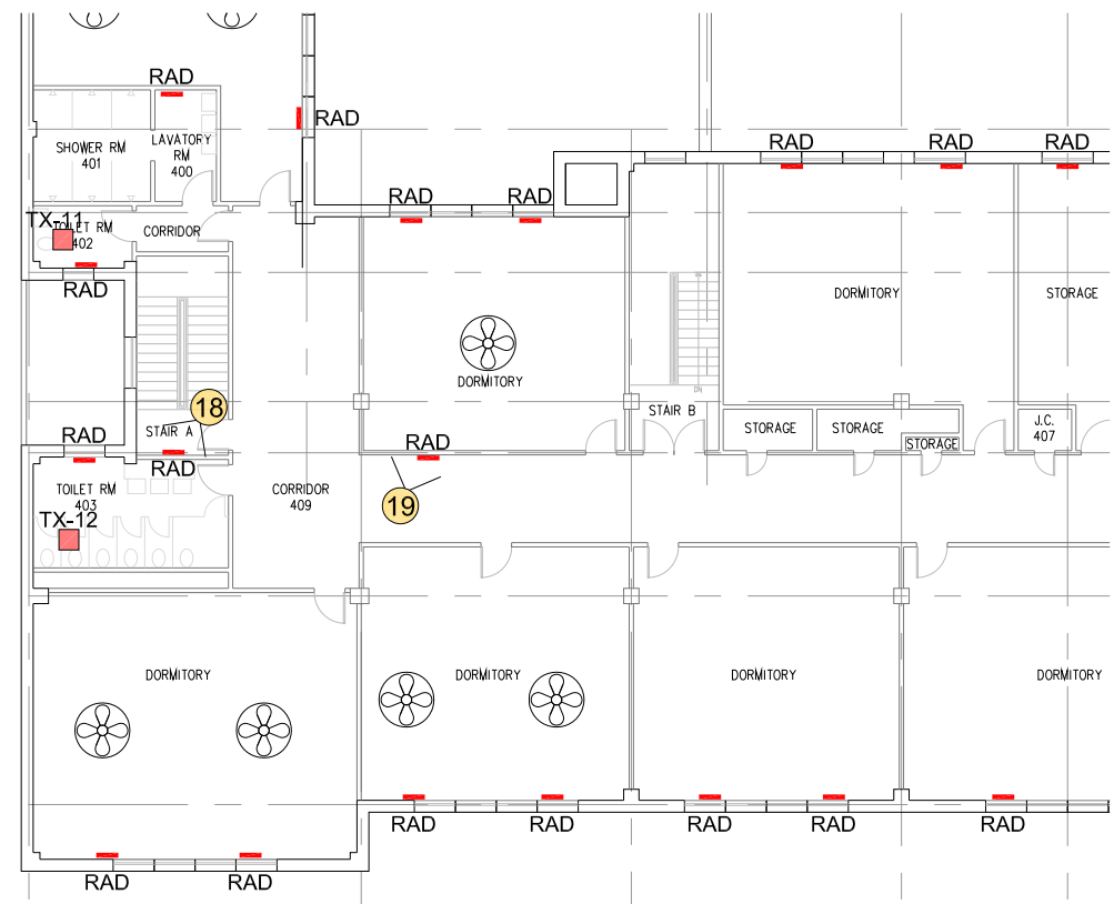
KEYPLAN (Partial 4th Floor Plan)
