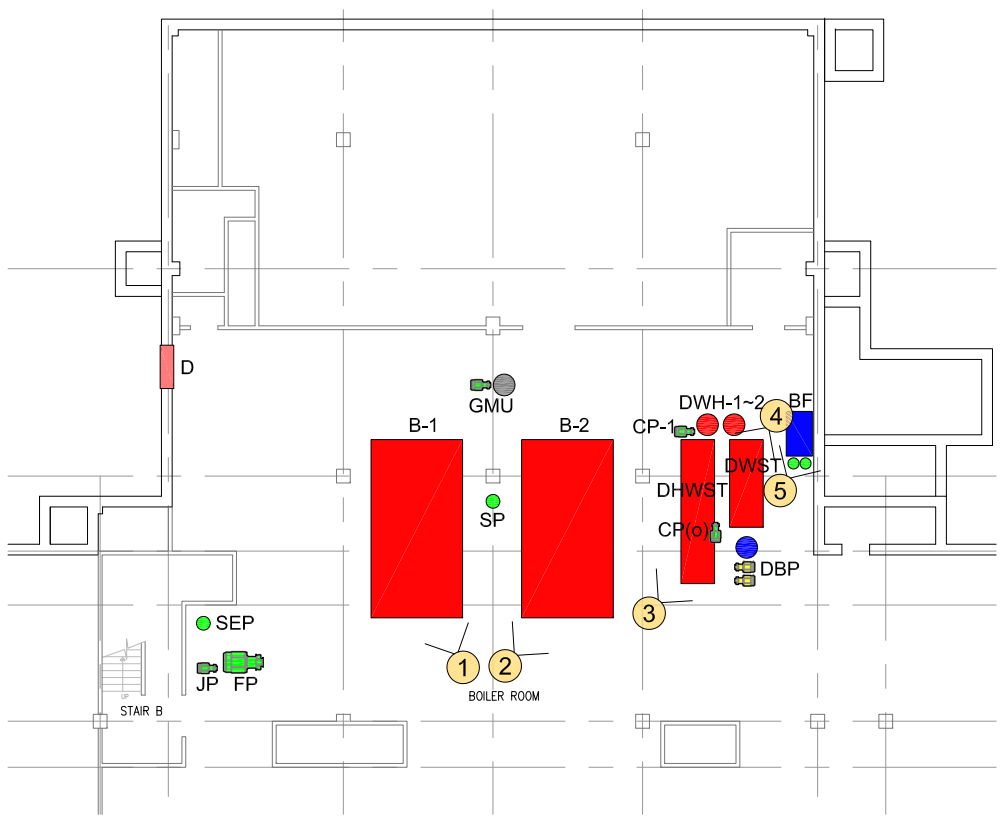
KEYPLAN (Partial Basement Floor Plan)
