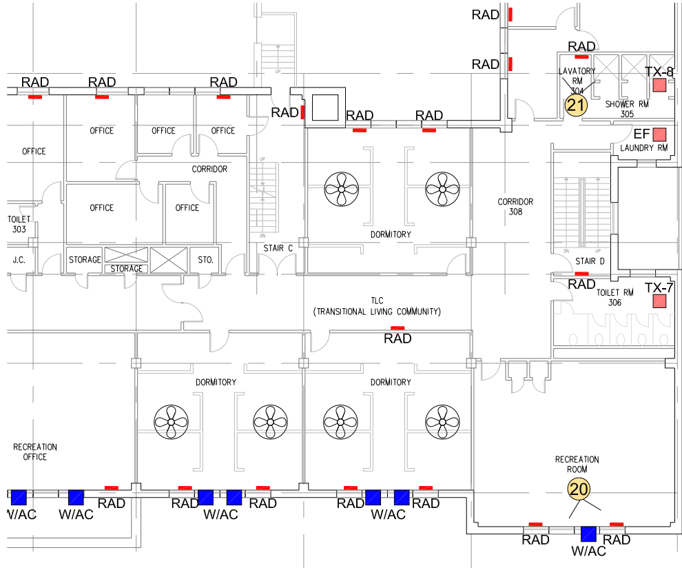
KEYPLAN (Partial 3rd Floor Plan)
